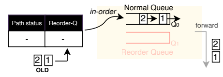
(a) Forwarding in-order packets to a normal queue.
