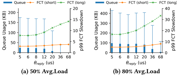
Figure 22: Avg/99-ile per-switch reorder queue usage and 99-ile FCT slowdowns for diverse \theta_{reply} in IRN RDMA. The smaller parameter makes a finer-grained rerouting.
