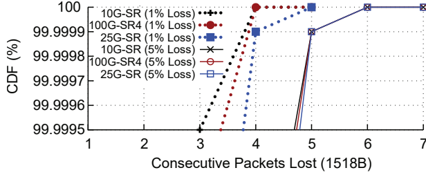
Figure 18: Distribution of consecutive packets lost.
