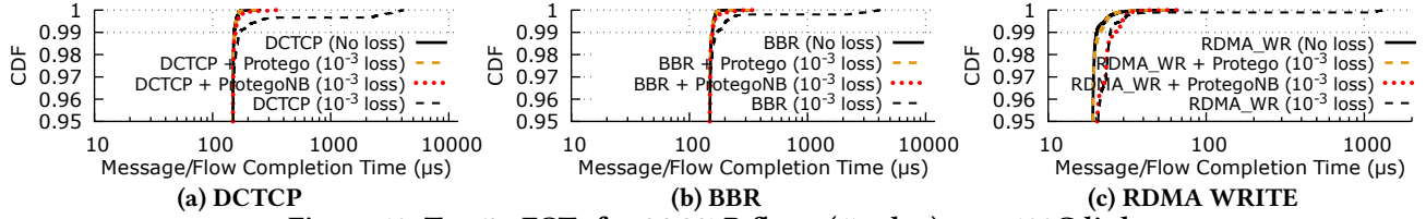
Figure 10: Top 5% FCTs for 24,387B flows (17 pkts) on a 100G link.
