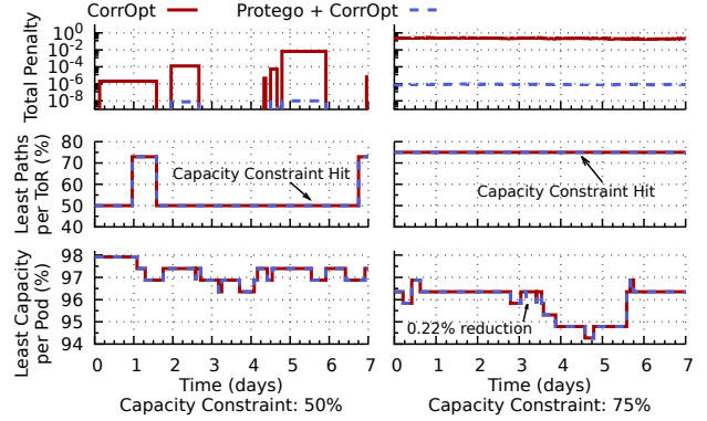
Figure 13: 1 week snapshot of simulation results for FB fabric topology (100K optical links).
