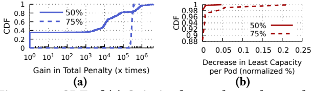
Figure 14: CDF of (a) Gain in the total penalty; and (b) Decrease in least capacity per pod; for Protego + Corropt compared to vanilla Corropt (1 year simulation).
