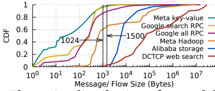
Figure 2: Flows size distribution of several datacenter workloads from 2008 to 2019 [3, 8, 34, 47, 50].
