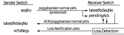
Figure 15: State maintained by Protego switches and different types of packets that read/update it.
