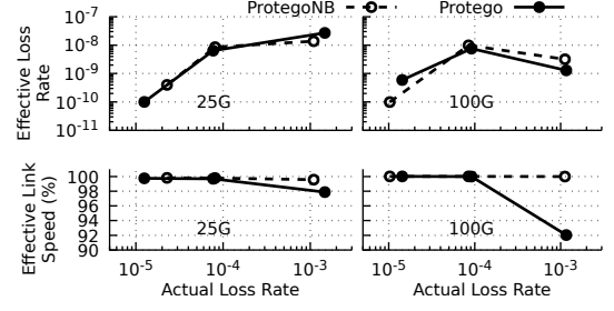
Figure 8: Effective loss rates achieved by Protego and the corresponding effective link speeds.
