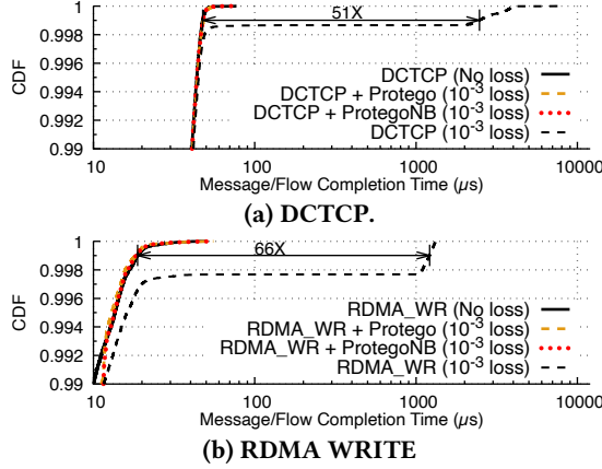
Figure 11: Top 1% FCTs for 143B flows on a 100G link.
