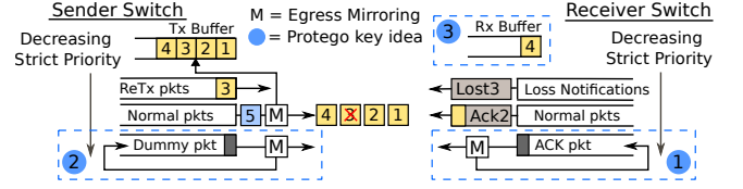
Figure 5: Protego Design Overview.
