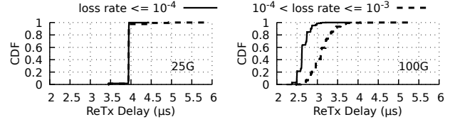
Figure 17: Delay observed by Protego receiver switch to receive retransmission from the time the loss was detected.
