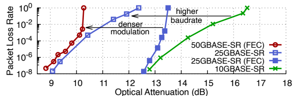
Figure 1: Effect of optical attenuation on various Ethernet link speeds (1518 B frames).
