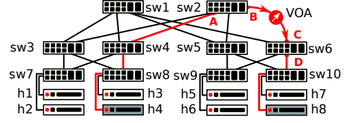
Figure 7: Testbed w/ Variable Optical Attenuator (VOA).
